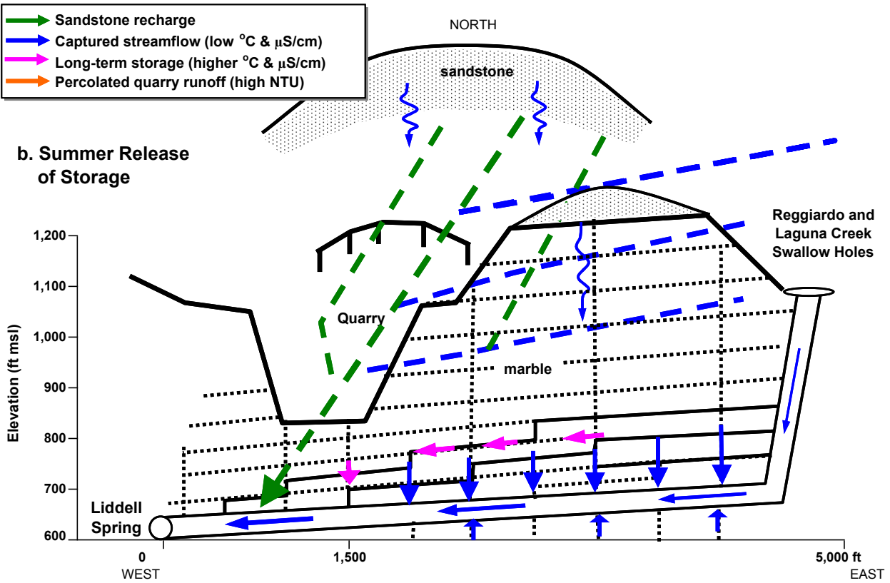
Conceptual Model of Seasonal Recharge and Storage Release from Marble Aquifer
